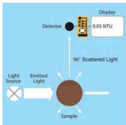
Principle of turbidity measurement.
